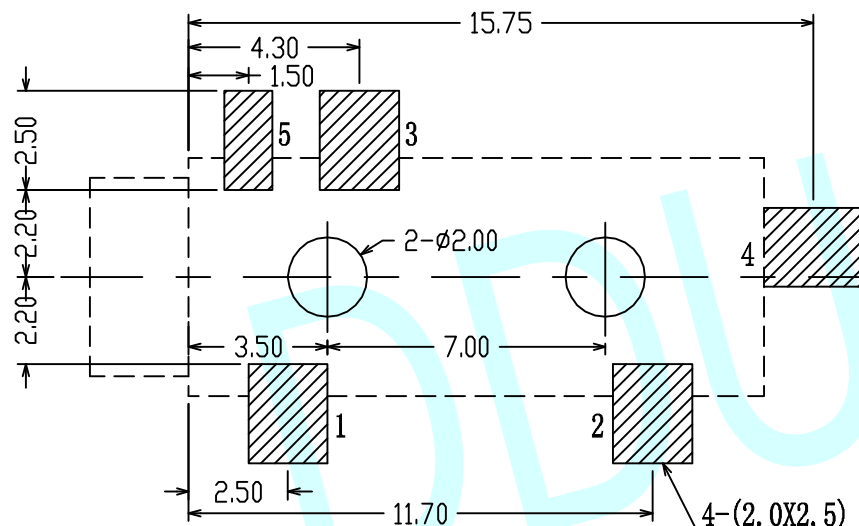
PCB Layout (Copper-Sided View)
