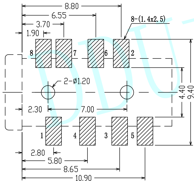
PCB Layout (Copper-Sided View)
