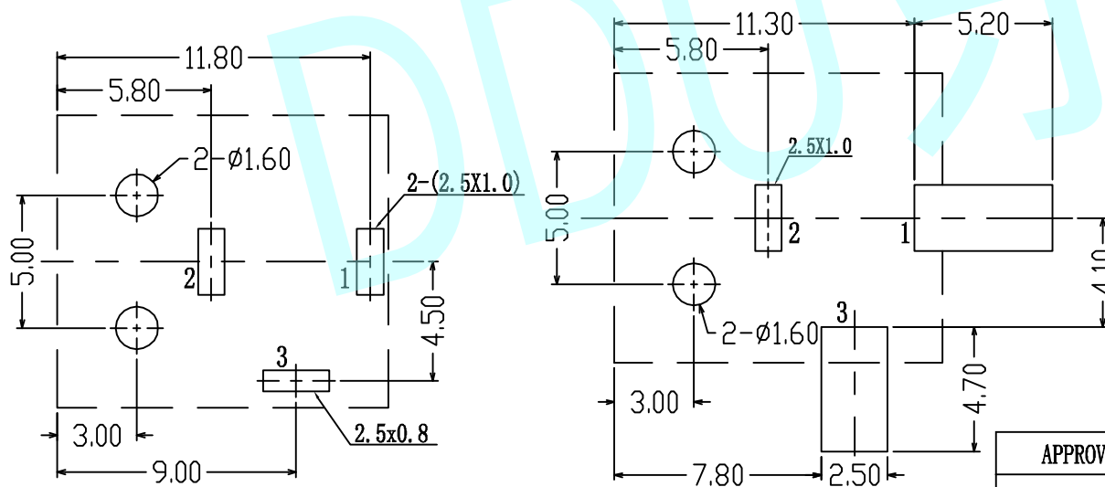
PCB Layout (Copper-Side View)
