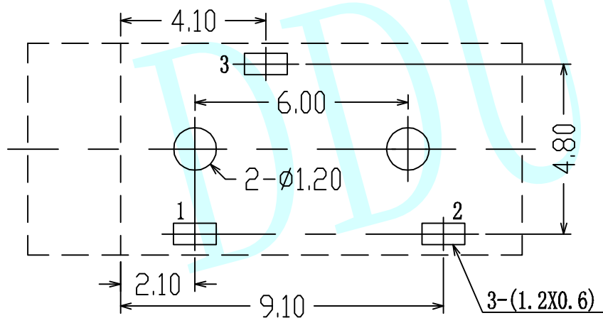
PCB Layout (Copper-Sided View)
