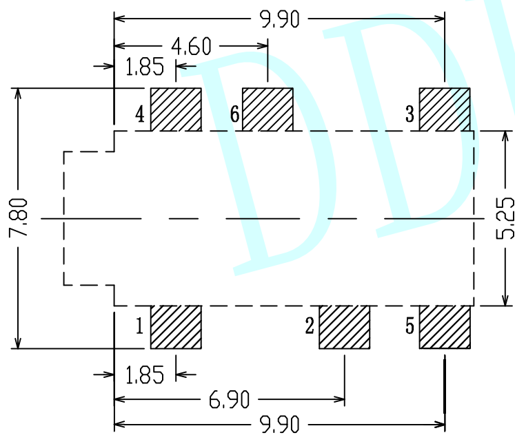
PCB Layout (Copper-Sided View)
