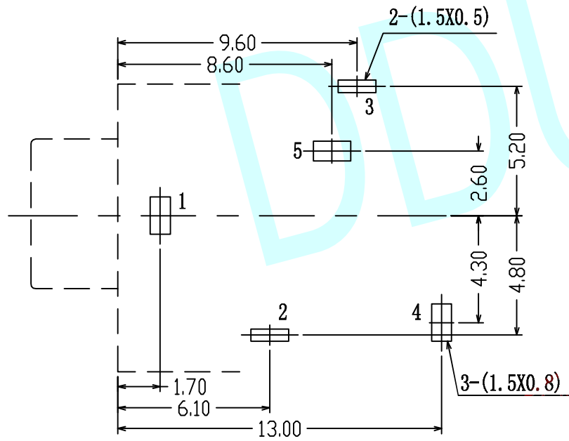
PCB Layout (Copper-Sided View)
