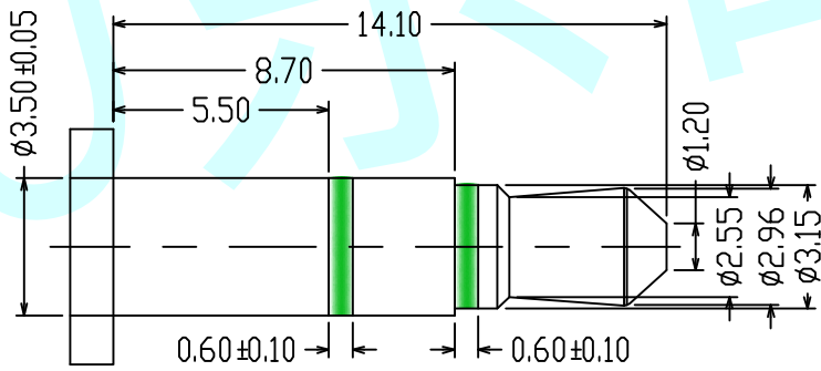
Matching Plug
