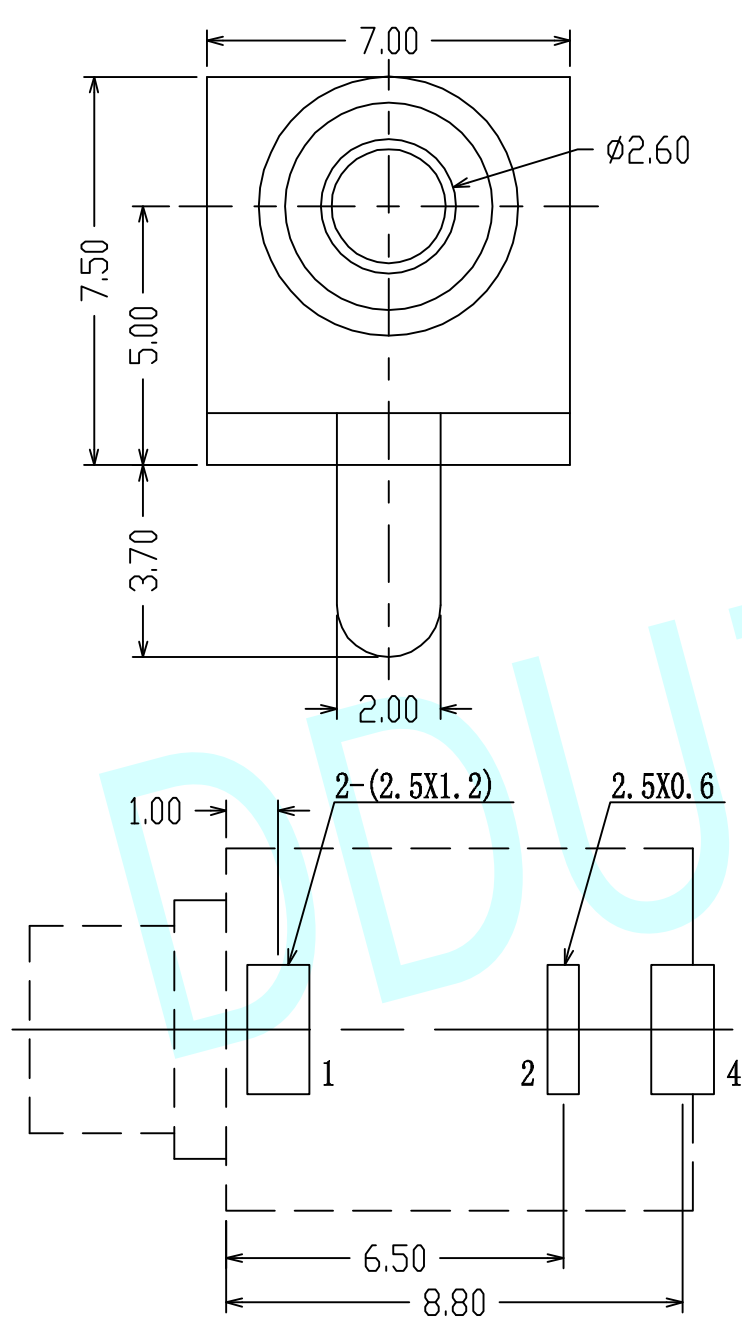
PCB Layout (Copper-Sided View)
