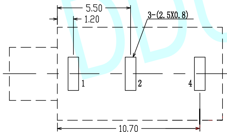
PCB Layout (Copper-Sided View)
