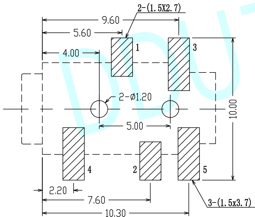
PCB Layout (Copper-Sided View)
