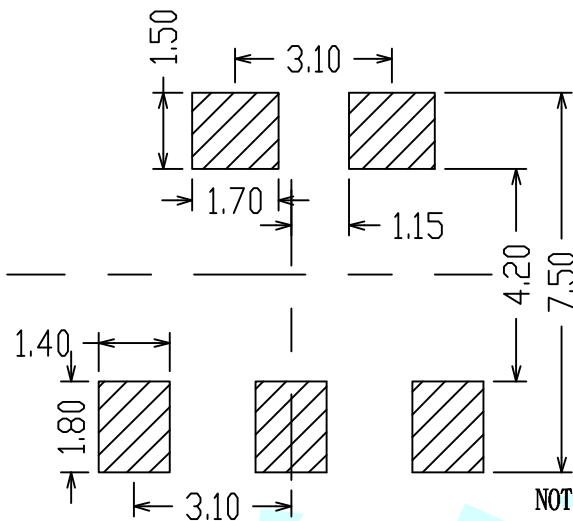
PCB Layout
