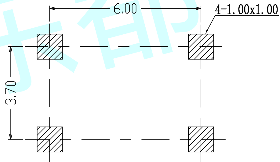
PCB Layout (Pattern Side)
