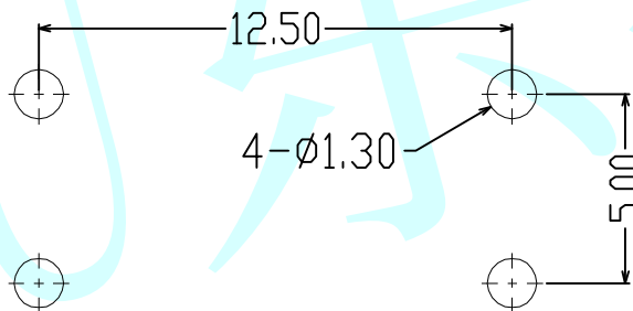
PCB Layout (Pattern Side)
